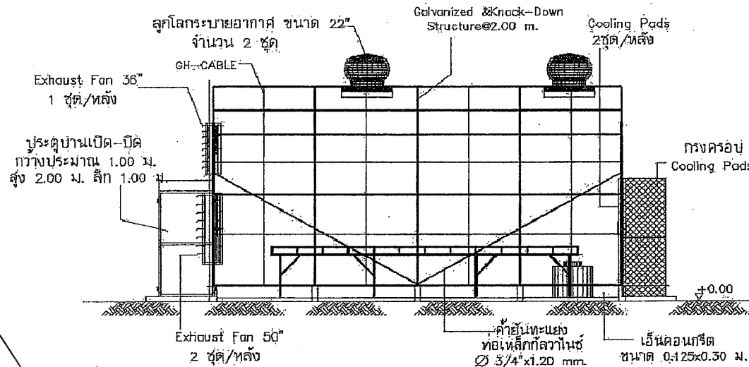
SIDE VIEW 1: 100
