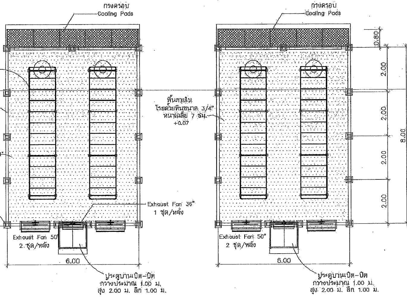
FLOOR PLAN 1: 100
