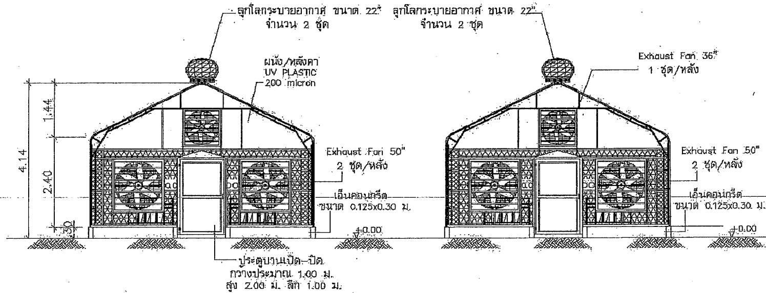
FRONT VIEW 1: 100
